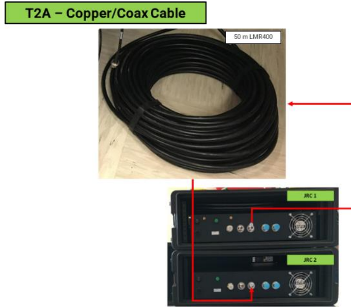
Figure 3-3: T2A Copper/Coax Cabled Timing Test Setup
