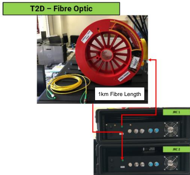
Figure 3-4: T2D Fibre Optic Cabled Timing Test Setup
