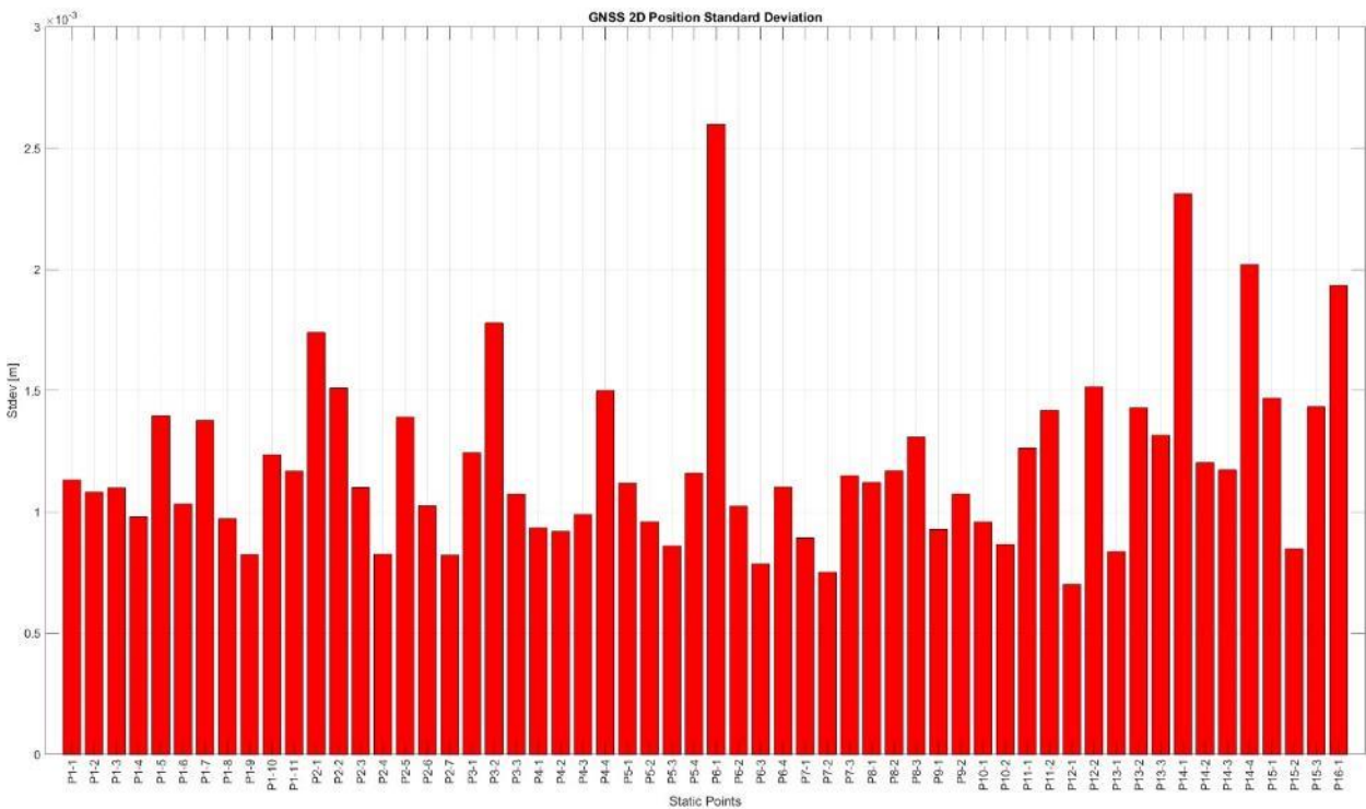
Figure 6-80: 2D Positioning Error Standard Deviations of the GNSS RTK Positioning Solutions for all Outdoor Static Occupations
