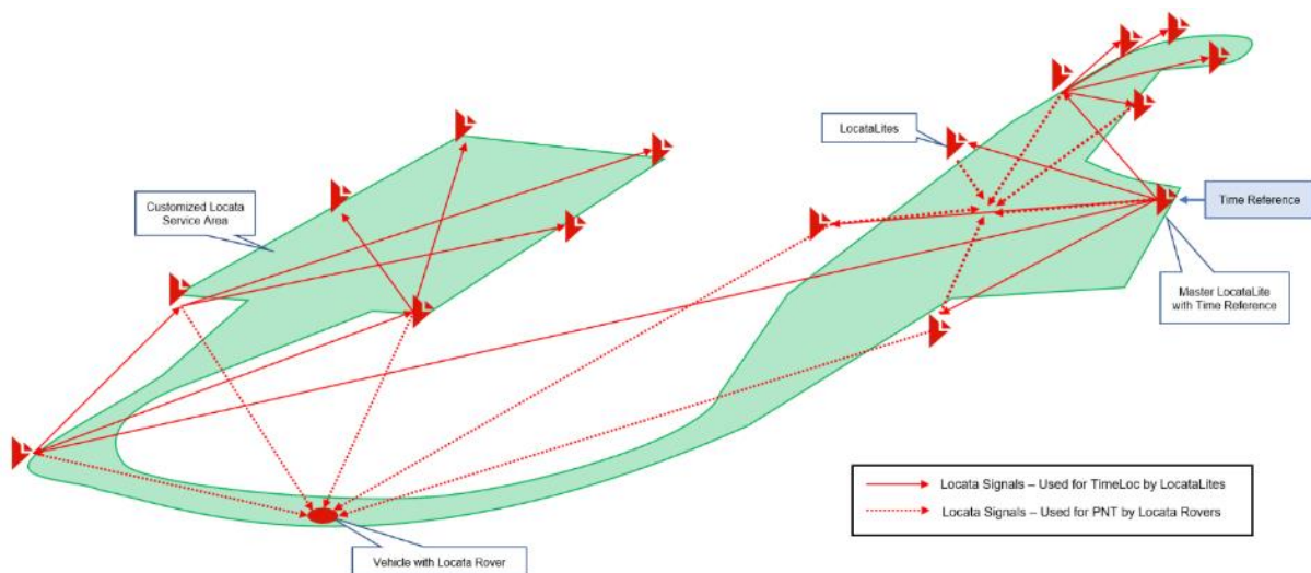
Figure 1-5: TimeLoc Time Synchronization in a LocataNet
