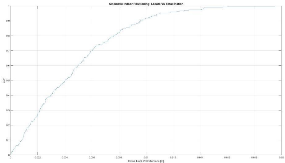
Figure 6-70: Cumulative Distribution Function for Kinematic Test Collection 1
