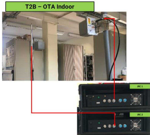
Figure 3-5: T2B OTA Indoor Timing Test Setup
