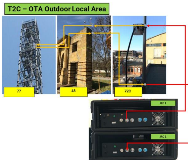
Figure 3-7: T2C OTA Outdoor Local Timing Test Setup
