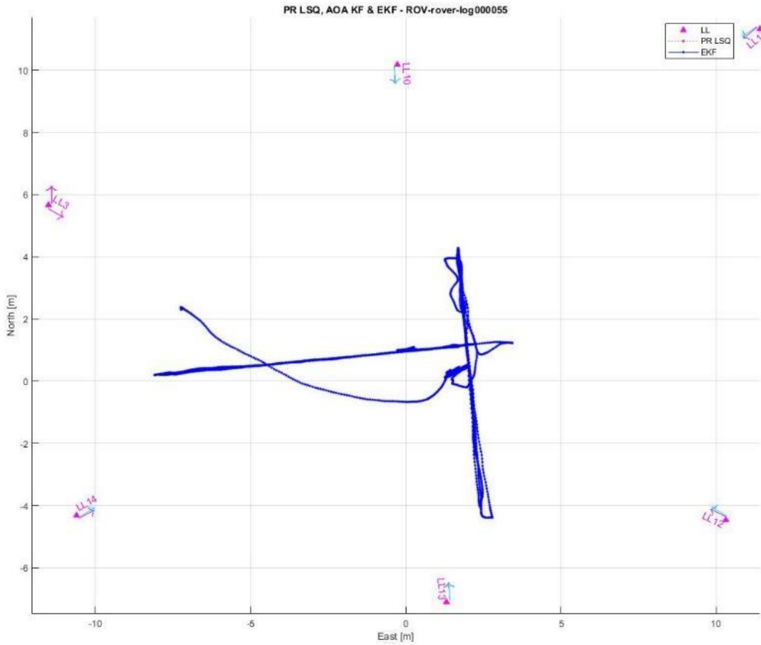
Figure 6-68: Locata Position Track for Kinematic Test Collection 2
