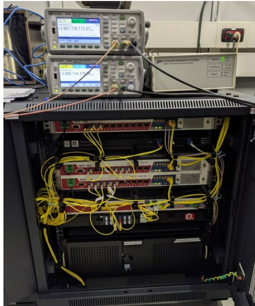
Figure 4. Example of JRC time rig setup for experiment
