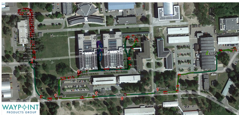
Figure 7. Example of kinematic test with visible permanent points
