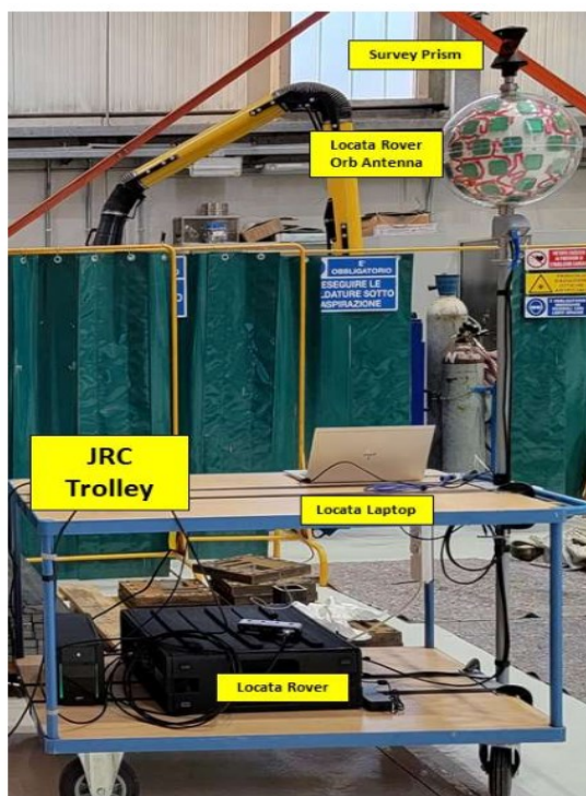
Figure 12. Indoor experiment set up
